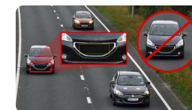
No-Plate Detection
